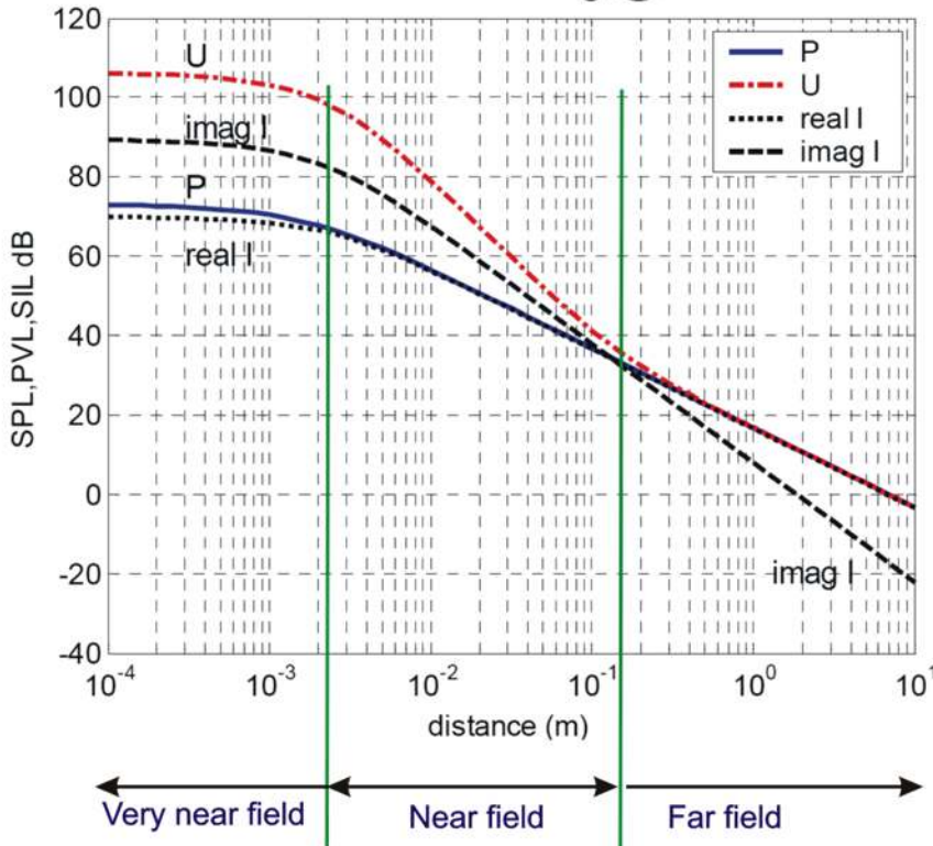
3 mm disc vibrating @ 400 Hz
