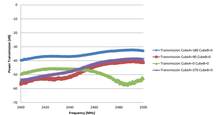
Figure 6: Transmission from satellite A to B in a reverberant room for different angles of satellite A
