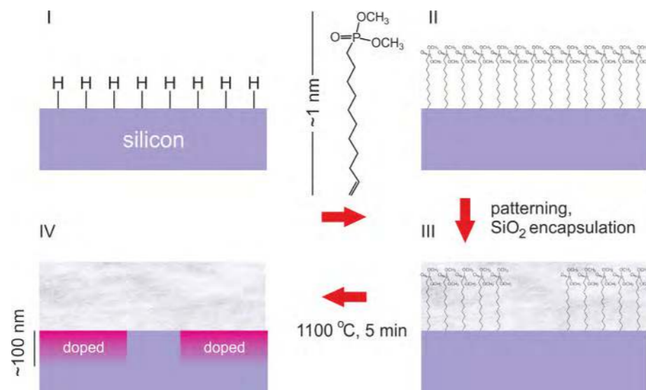
Figure 1: Schematic representation of molecular layer doping of silicon (not to scale) I: The natural \text{SiO}_2 is removed by \text{NH}_4 and a hydrogen-terminated ( \text{Si-H} ) surface is created. II: A full monolayer of molecules (1-undecenyl-dimethylphosphonate) containing the donor atom phosphorus (P). III: Nano imprint lithography combined with an oxygen plasma etch is used to pattern the monolayer at the micronscale. After that, the patterned monolayer is encapsulated in \text{SiO}_2 to prevent loss of the molecules in the subsequent thermal in-diffusion step. IV: During this last step the molecules fully disintegrate and the P atoms diffuse (partly) into the silicon [1].
