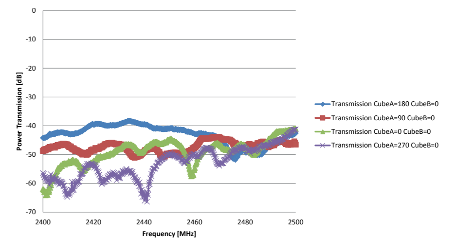
Figure 7: Transmission from satellite A to B in the anechoic chamber for different angles of satellite A
