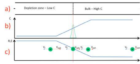
Figure 11. Schematic representation of depletion zone isotachopheresis
