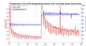
Figure 6. Step response of the control loop showing the temperature at Heater 1 and the duty cycle controlling the power in Heater 1. After 18 seconds the set point was changed from 50°C to 75°C.
