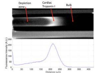
Figure 12. Dz-ITP of 100 ng/L of fluorescent cTn-I in phosphate buffered saline. Top: Fluorescent image microscopy image take after 2 min. Bottom: Fluorescent intensity profile. The fluorescent intensity corresponds to cTn-I concentration. As show in the profile, the bulk concentration of cTn-I is practically 0 A.U. and after 2 min it has increased more than 200 A.U.
